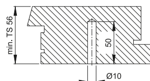
houten-profiel
