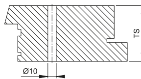
houten-profiel
