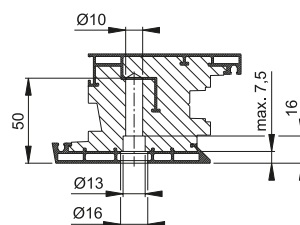
pural-profiel
