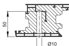
pural-profiel
